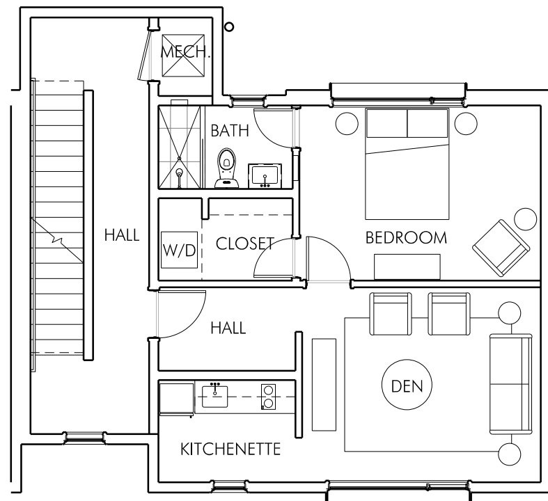
2ND FLOOR
