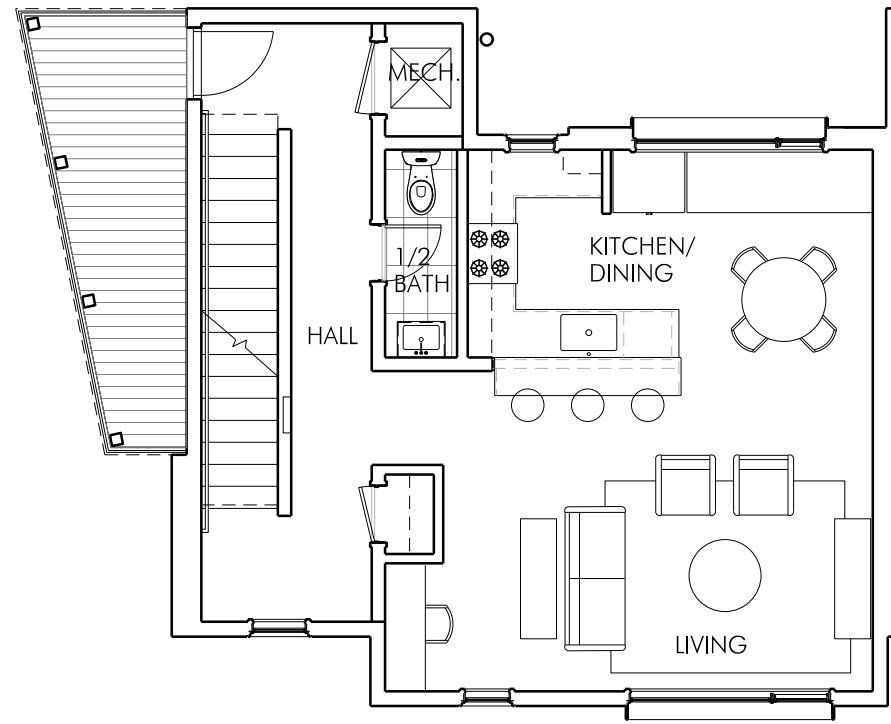
THIRD FLOOR
