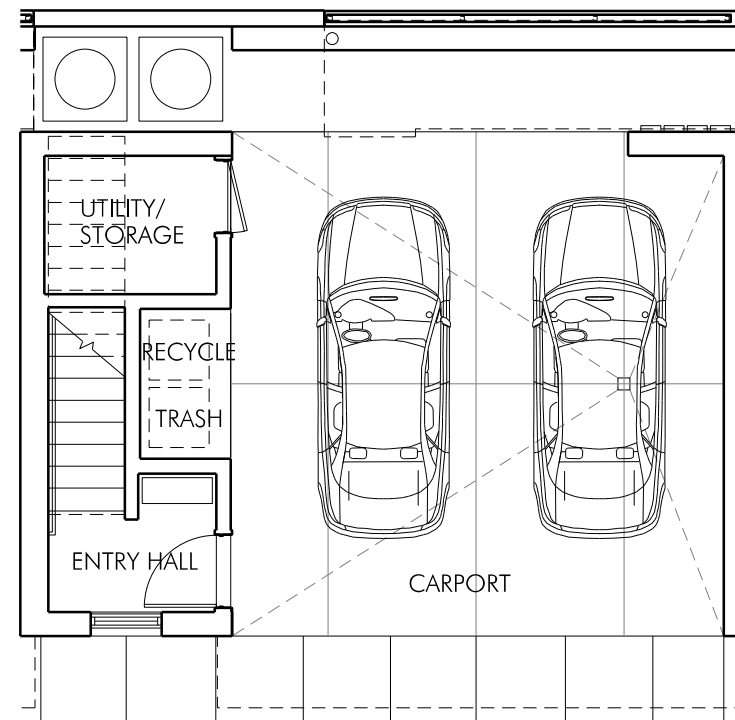
GARAGE/ ENTRY
