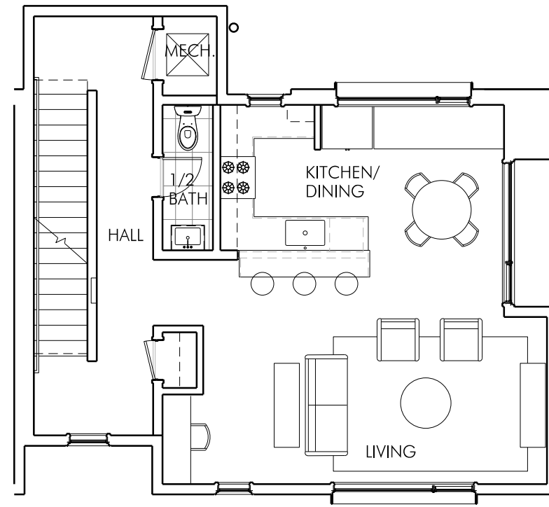
THIRD FLOOR
