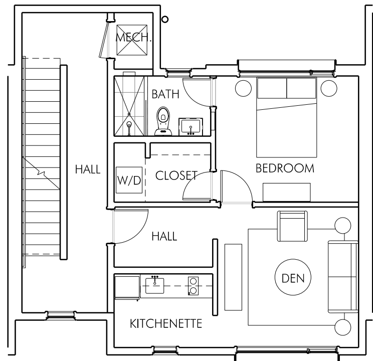
2ND FLOOR
