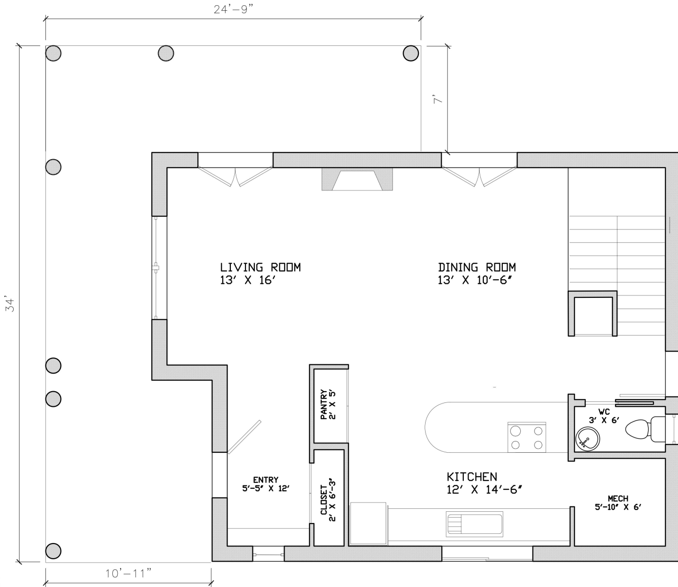
① FIRST FLOOR PLAN SCALE: 1/4" = 1'0"
