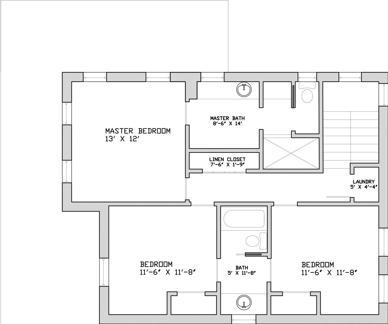
1 SECOND FLOOR PLAN SCALE: 1/4" = 1'0"
