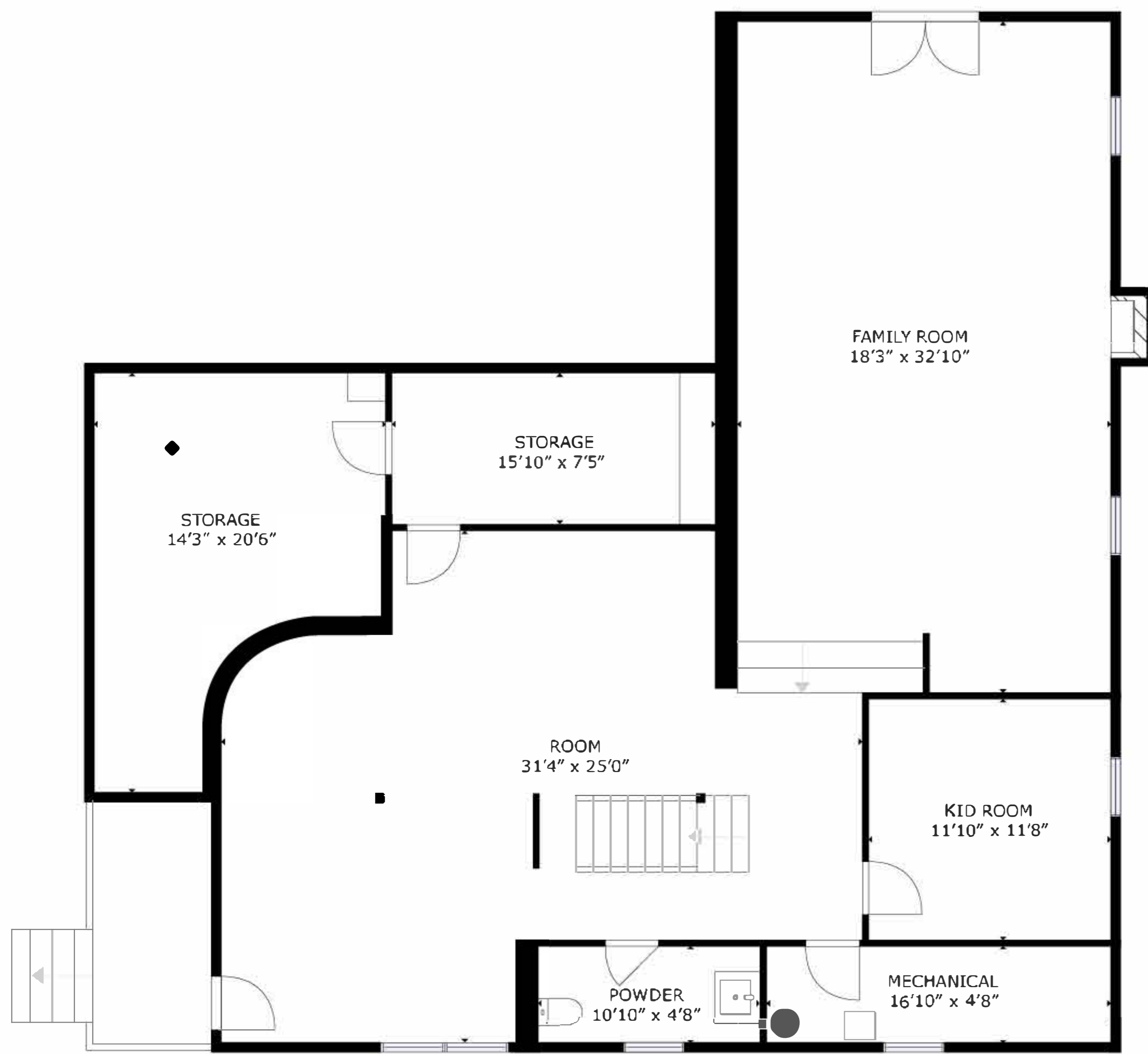
BASEMENT 1
