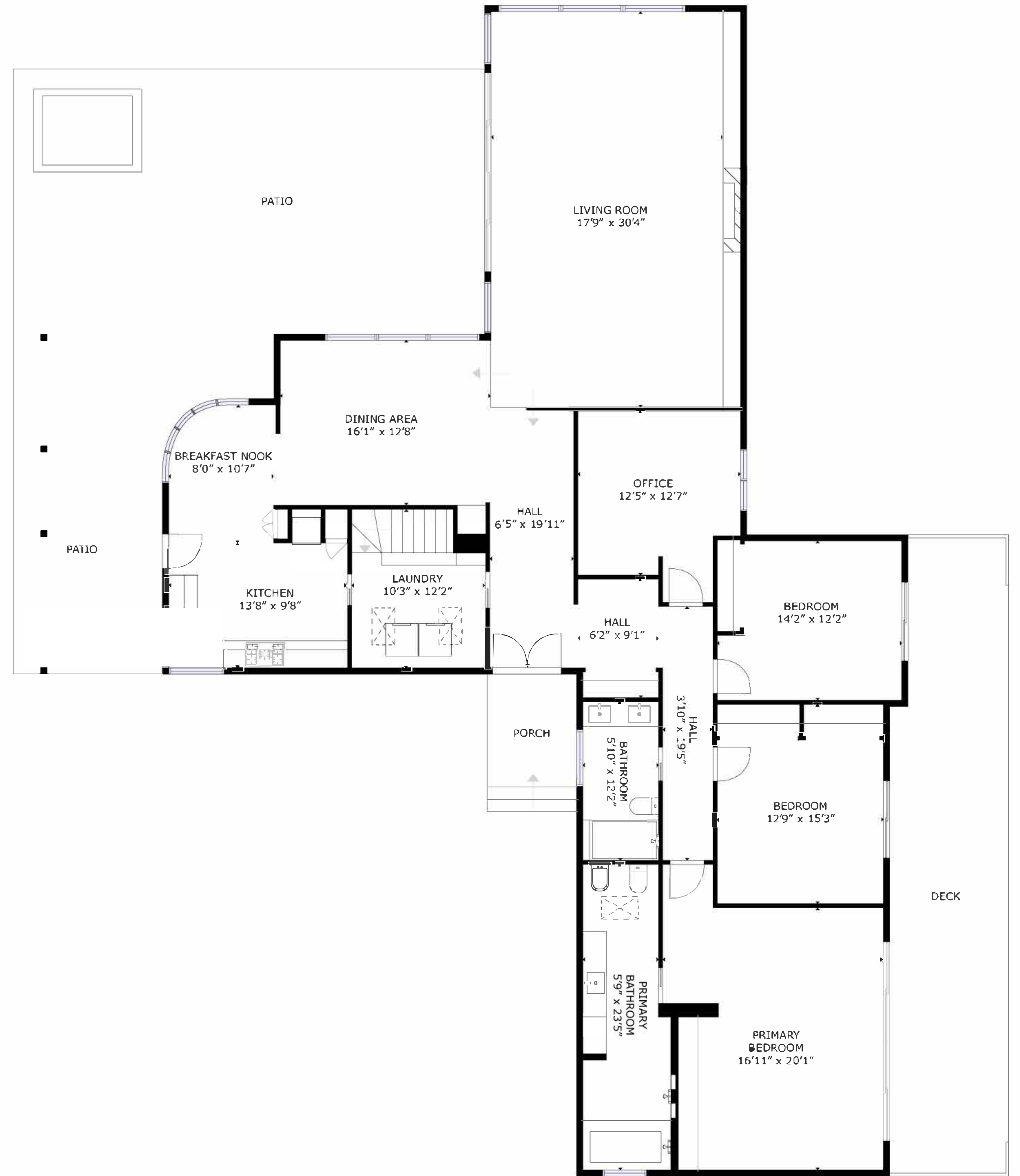
FLOOR 1
