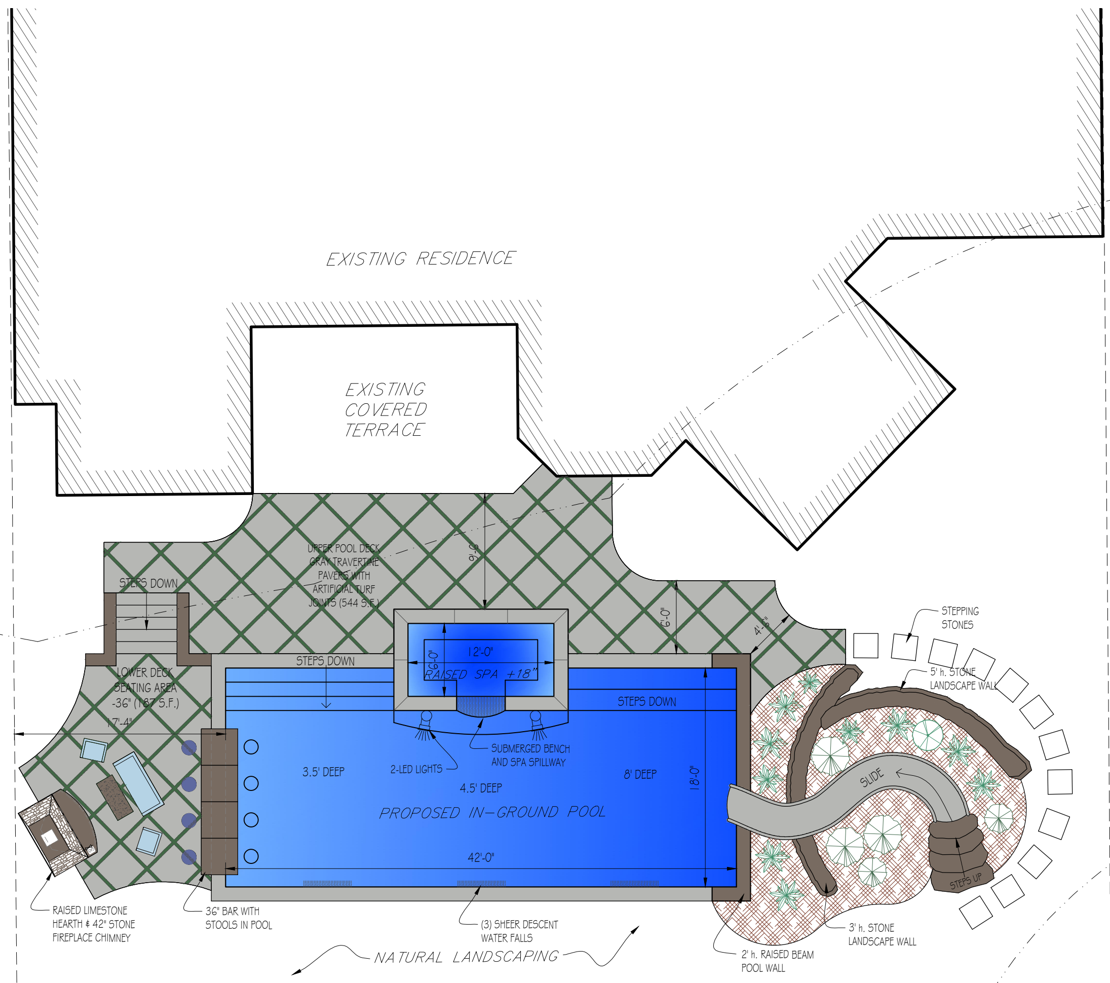
POOL PLAN SCALE 1/8" = 1'-0"
