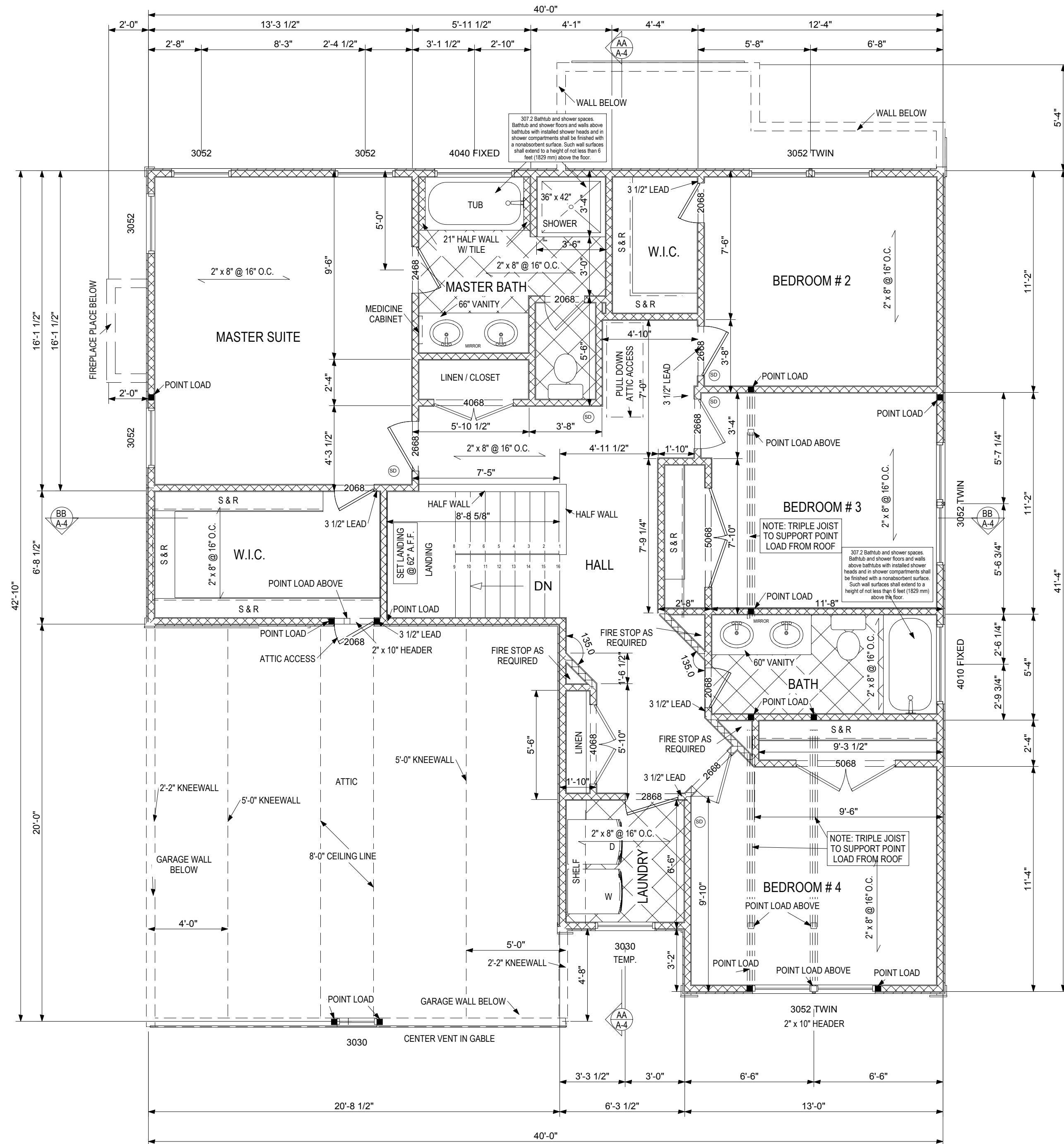
SECOND FLOOR
