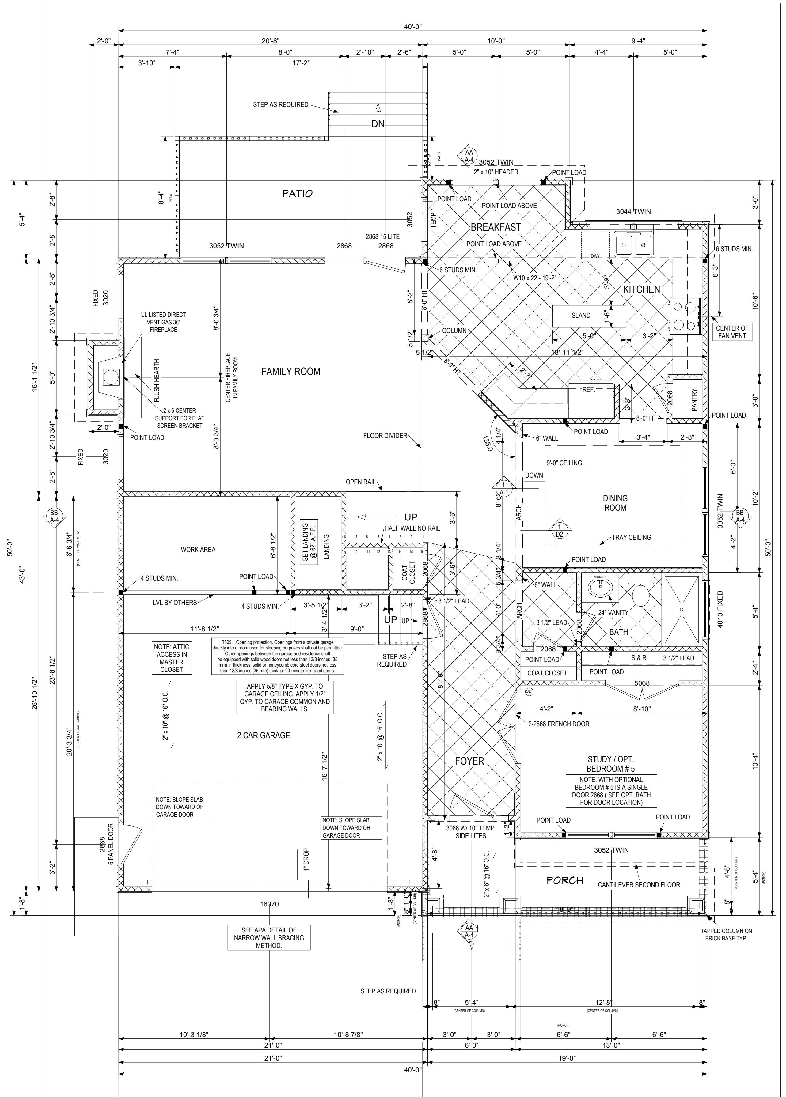
FIRST FLOOR
