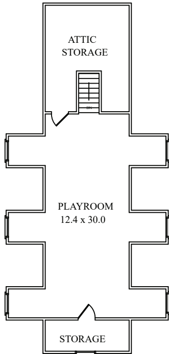
SECOND FLOOR OVER GARAGE
