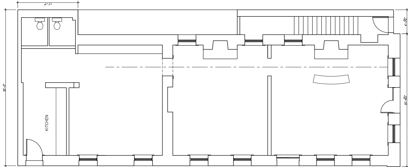
FIRST FLOOR PLAN option 3 OFFICE AREA 1503 SQ.FT. STAIR WELL 100 SQ. FT.
