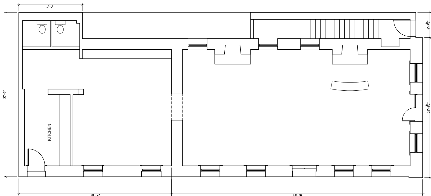
FIRST FLOOR PLAN option 1 OFFICE AREA 1503 SQ.FT. STAIR WELL 100 SQ. FT.
