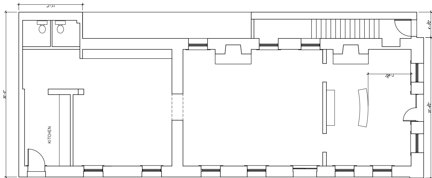
FIRST FLOOR PLAN option 2 OFFICE AREA 1503 SQ.FT. STAIR WELL 100 SQ. FT.
