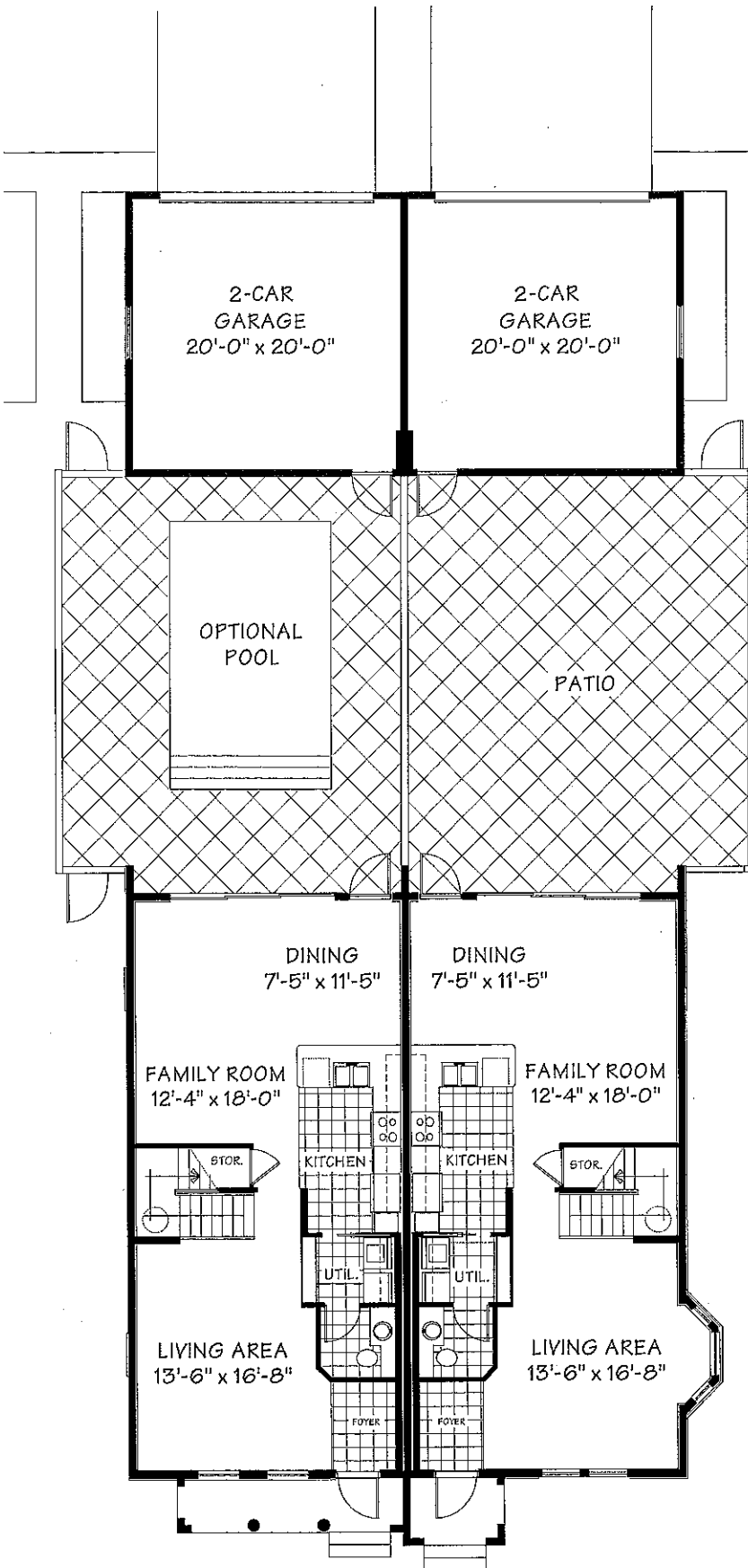
FIRST FLOOR
