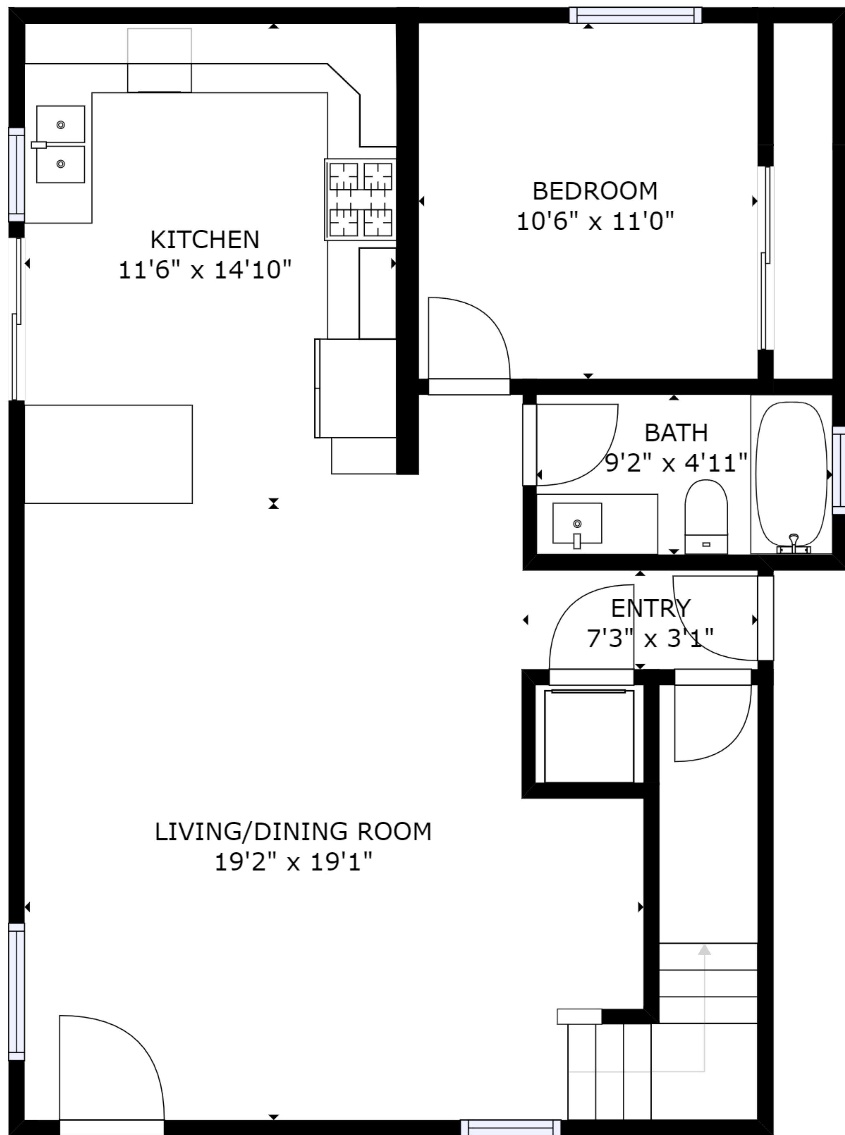
FLOOR 1
